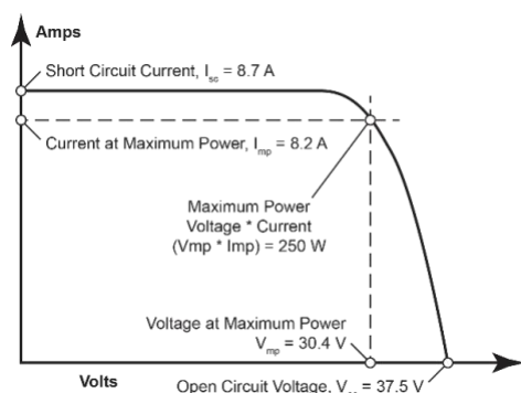
Figure 5: I-V curve of a solar panel
