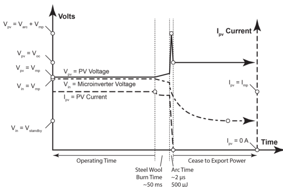
Figure 5: I-V curves explaining the microinverter behaviour during an Arc Fault
