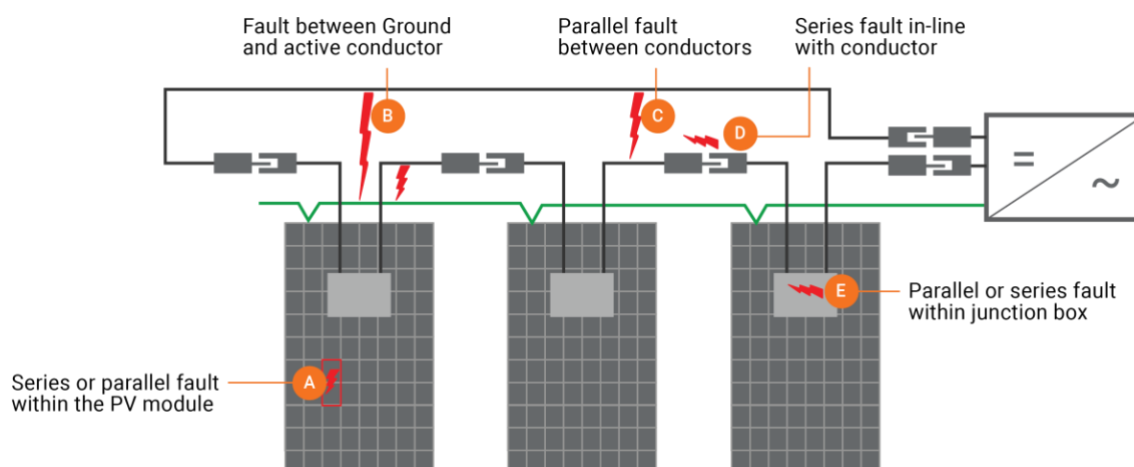
Figure 4: Different Arc Fault possibilities in a typical String Inverter system
