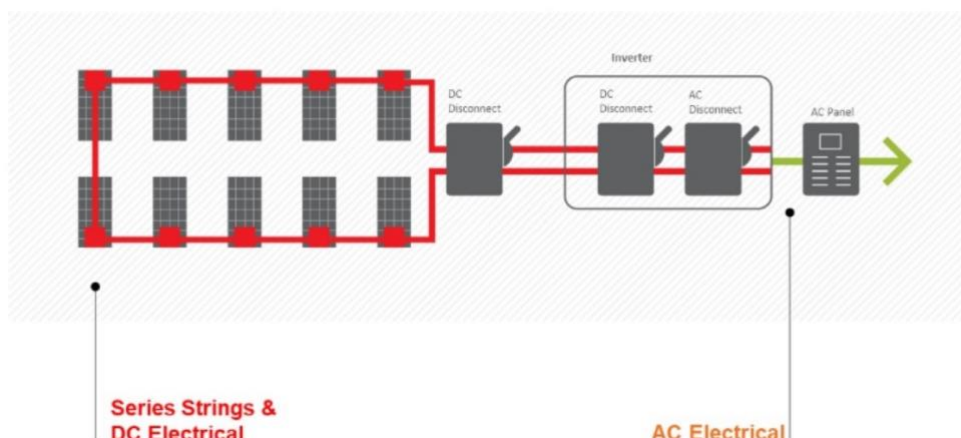
Figure 2: A typical DC String Inverter system with both Rooftop and Inverter DC Isolators
