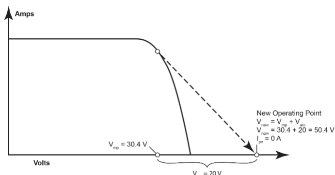
Figure 6: With an arc-fault in series with a working microinverter, the voltage rises to V_{mp} + V_{arc} . The transfer characteristic of the PV Panel forces the current to zero. With zero current, the microinverter falls off MPPT (Maximum Power Point Tracking) and shuts down.
